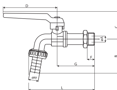
DN 25
